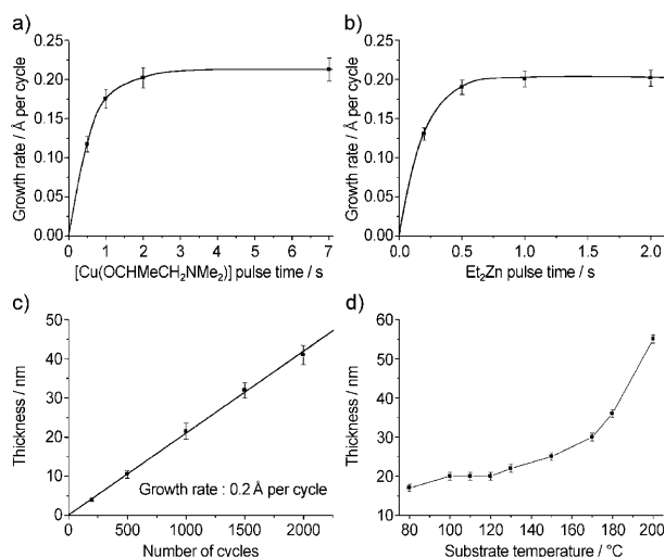
Figure 1. Growth rate a) as a function of [\text{Cu}(\text{dmap})_2] pulse time, b) as a function of \text{Et}_2\text{Zn} pulse time for copper films grown at 100–120 °C. Thickness of the copper films c) versus the number of ALD cycles at 100–120 °C, d) versus the substrate temperature.
