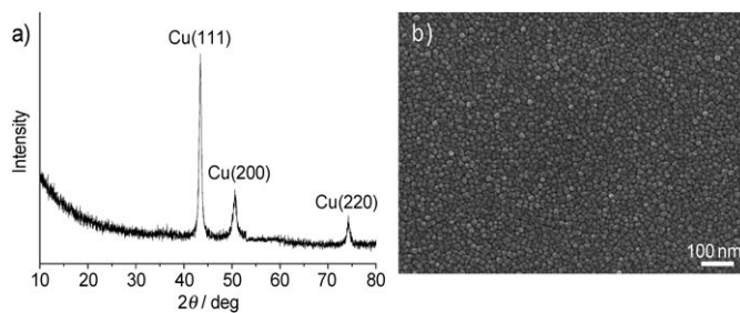
Figure 3. a) XRD pattern, b) SEM image of the copper thin films grown at 100–120 °C.
