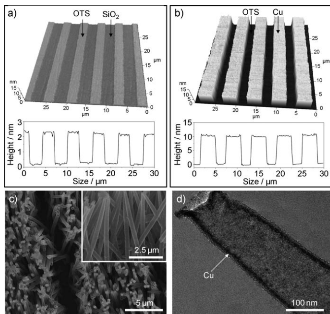
Figure 4. AFM image and cross-section a) of the patterned OTS-SAMs fabricated by microcontact printing on Si substrates, b) of the patterned Cu thin film produced using selective ALD on SAMs-patterned Si substrates. c) Field-emission SEM images of Cu nanotubes. d) HR-TEM image of a Cu nanotube.
