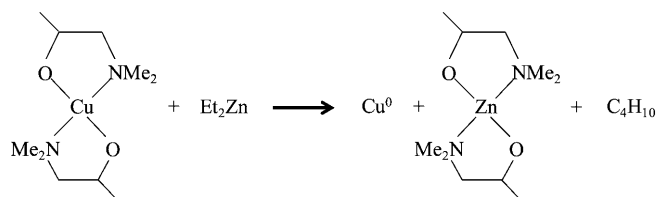
Scheme 1. Reaction between [Cu(dmap) 2 ] and Et 2 Zn.
