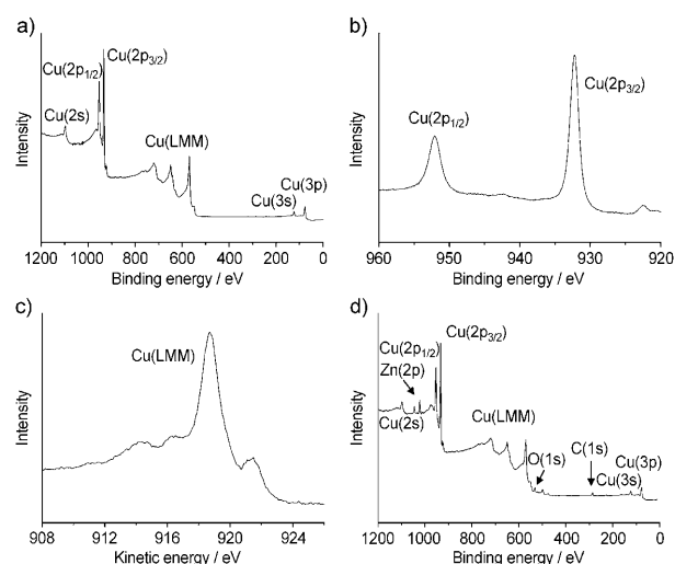
Figure 2. Spectra of the copper films grown at 100–120 °C: a) Survey XP spectrum; b) high-resolution XP spectrum of the \text{Cu}(2p) regions; c) Auger spectrum of the \text{Cu}(\text{LMM}) regions. d) Survey XP spectrum for the copper films grown at 130 °C.
